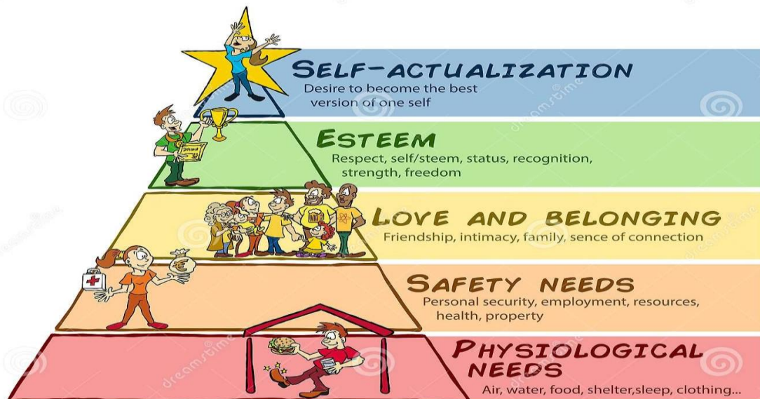
PSLES Model
